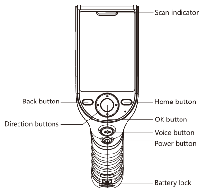
Fig. 1 Front view
