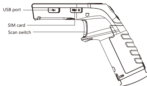
Fig. 2 Left view
